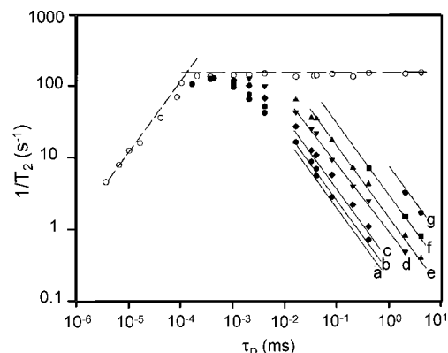
Figure 15. Computer-generated data for spheres with v = 5 \times 10^{-6} and \Delta\omega_r = 2.36 \times 10^7 rad/s, plotted versus \tau_D . The open symbols represent the 1/T_2^* value, while the filled symbols represent the rates obtained, respectively, with \tau_{CP} = 0.1 ms (● and line a), 0.2 ms (● and line b), 0.5 ms (◆ and line c), 2 ms (▼ and line d), 5 ms (▲ and line e), 10 ms (■ and line f), 20 ms (● and line g). The short dashed line is the rate predicted by the outer sphere theory (eq 30), and the long dashed line is the static dephasing relaxation model given in ref 584. Lines a–g are the rates given by eq 34.
